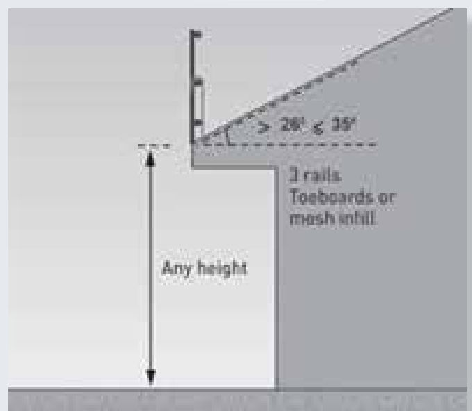
Roof pitch greater than 26°.
